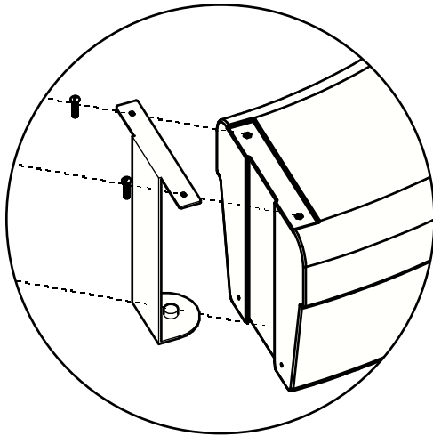
DETAIL: A END CAP CONNECTION DETAIL
