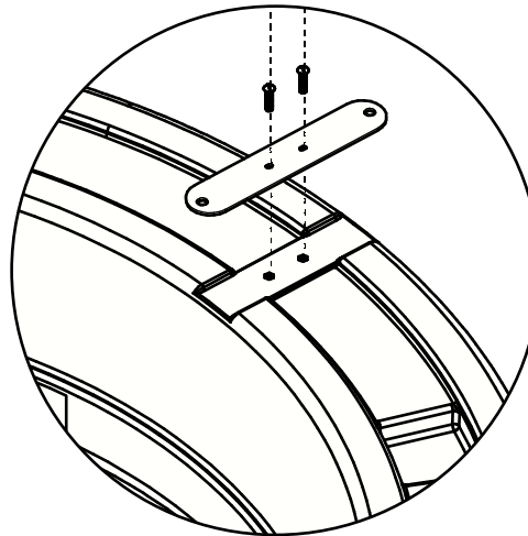
DETAIL: B MOUNTING PLATE CONNECTION DETAIL
