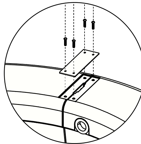
DETAIL: D TOP CONNECTOR CONNECTION DETAIL
